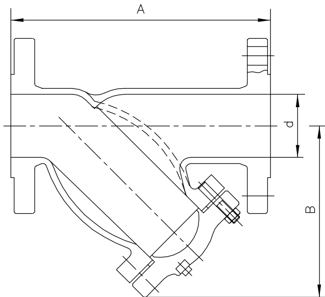
PN10 Fig No.51010 DIMENSIONS AND WEIGHTS
