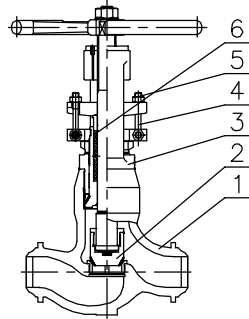
GLOBE VALVES
