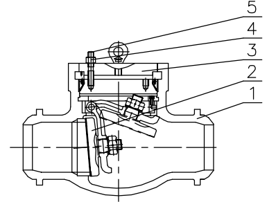
CHECK VALVES
