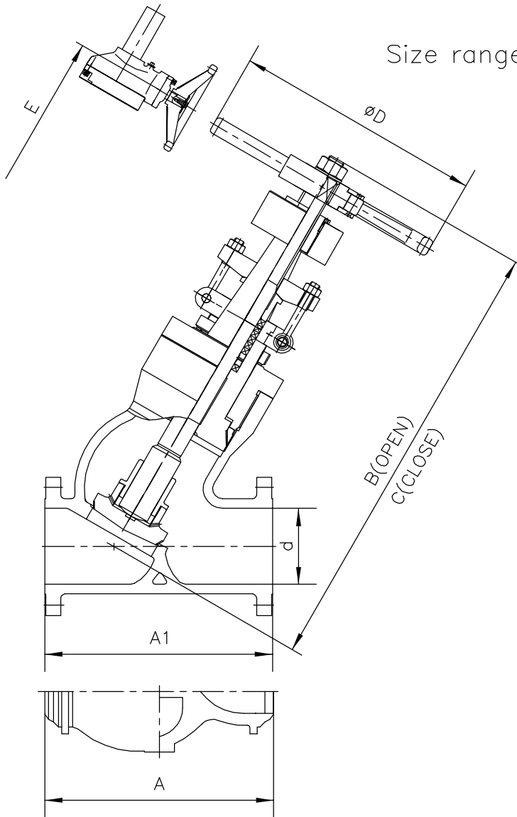
Class 1500# FIG 61500 PSY DIMENSIONS AND WEIGHTS
