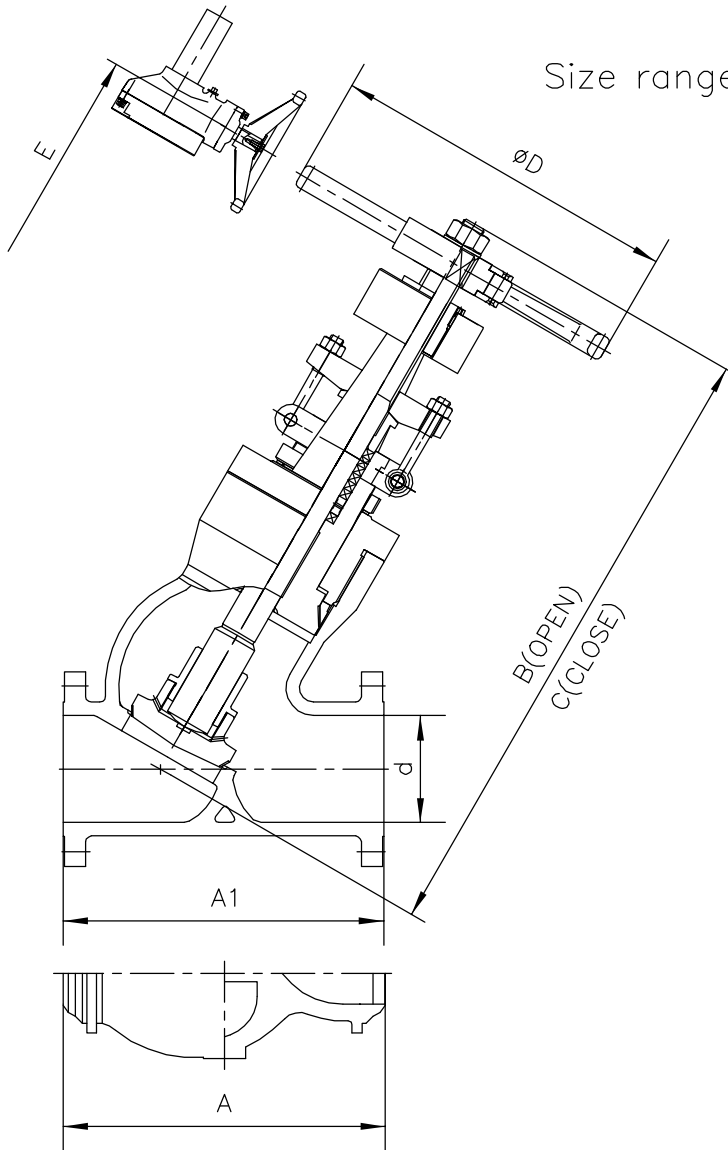
Class 600# FIG 6600 PSY DIMENSIONS AND WEIGHTS
