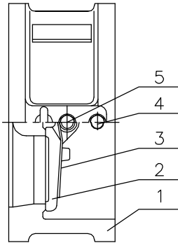
WAFER CHECK VALVES
